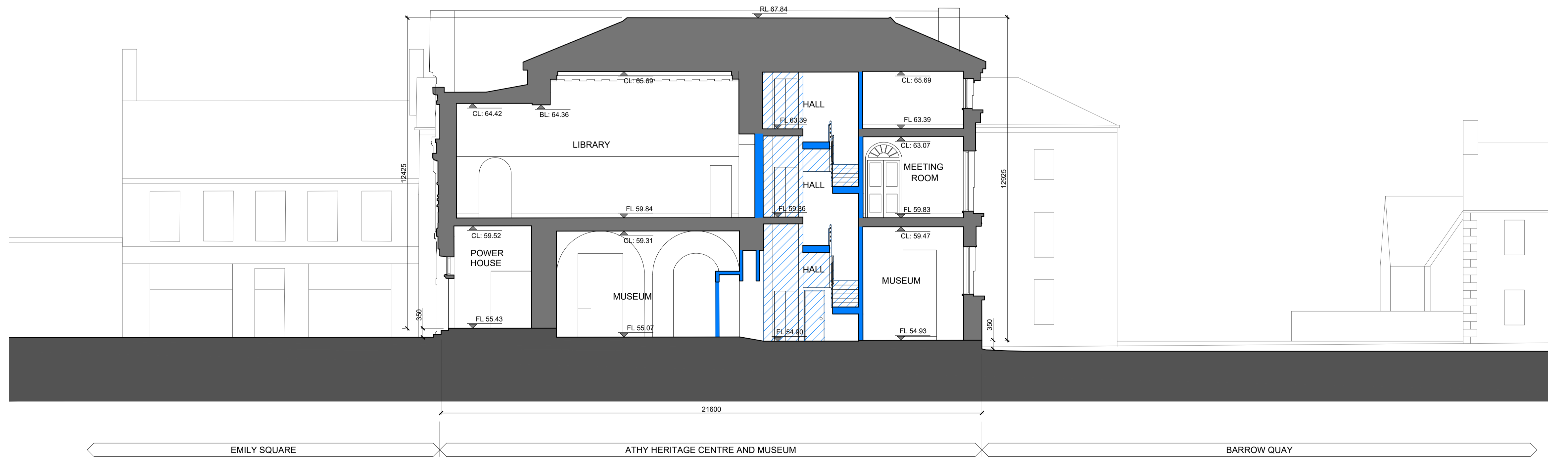
2 EXISTING SECTION B-B 1:100QA1, 1:200QA3
